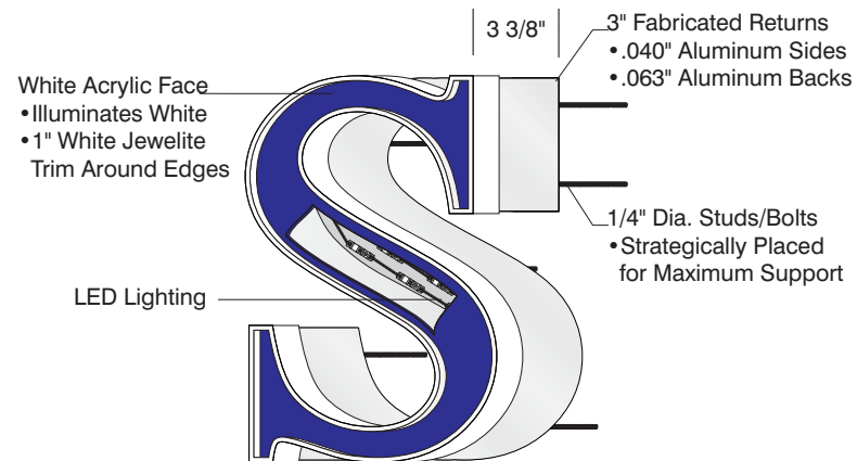
LED Illuminated Wall Mounted Typical Channel Letter Detail
