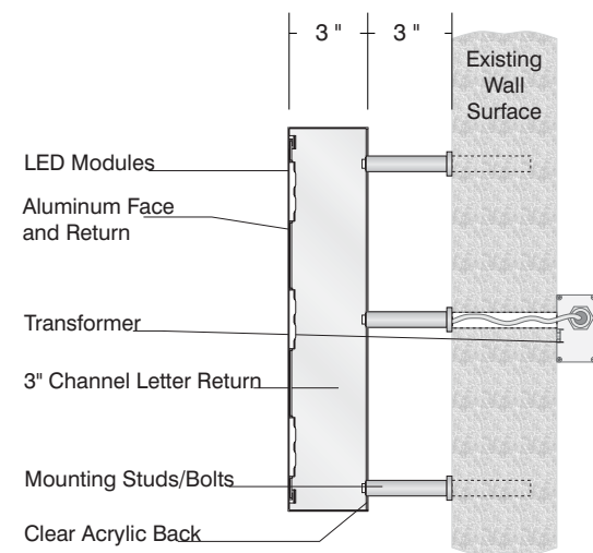
Wall Mounted Reverse Lit Channel Letter Cross Section Detail
