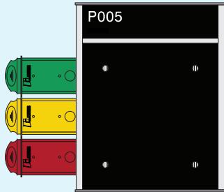
STANDARD TABS FINGOOD: HIDPFH-F8511-3 MINIMUM WALL CLEARANCE: 14"
