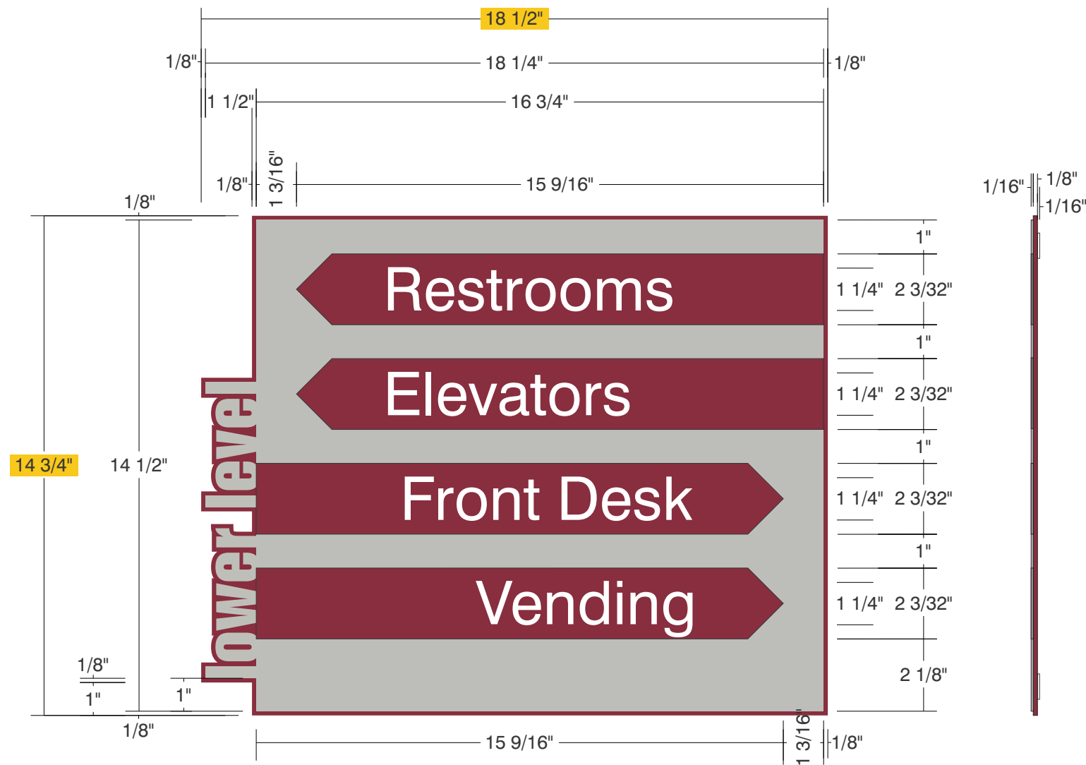
Front View
