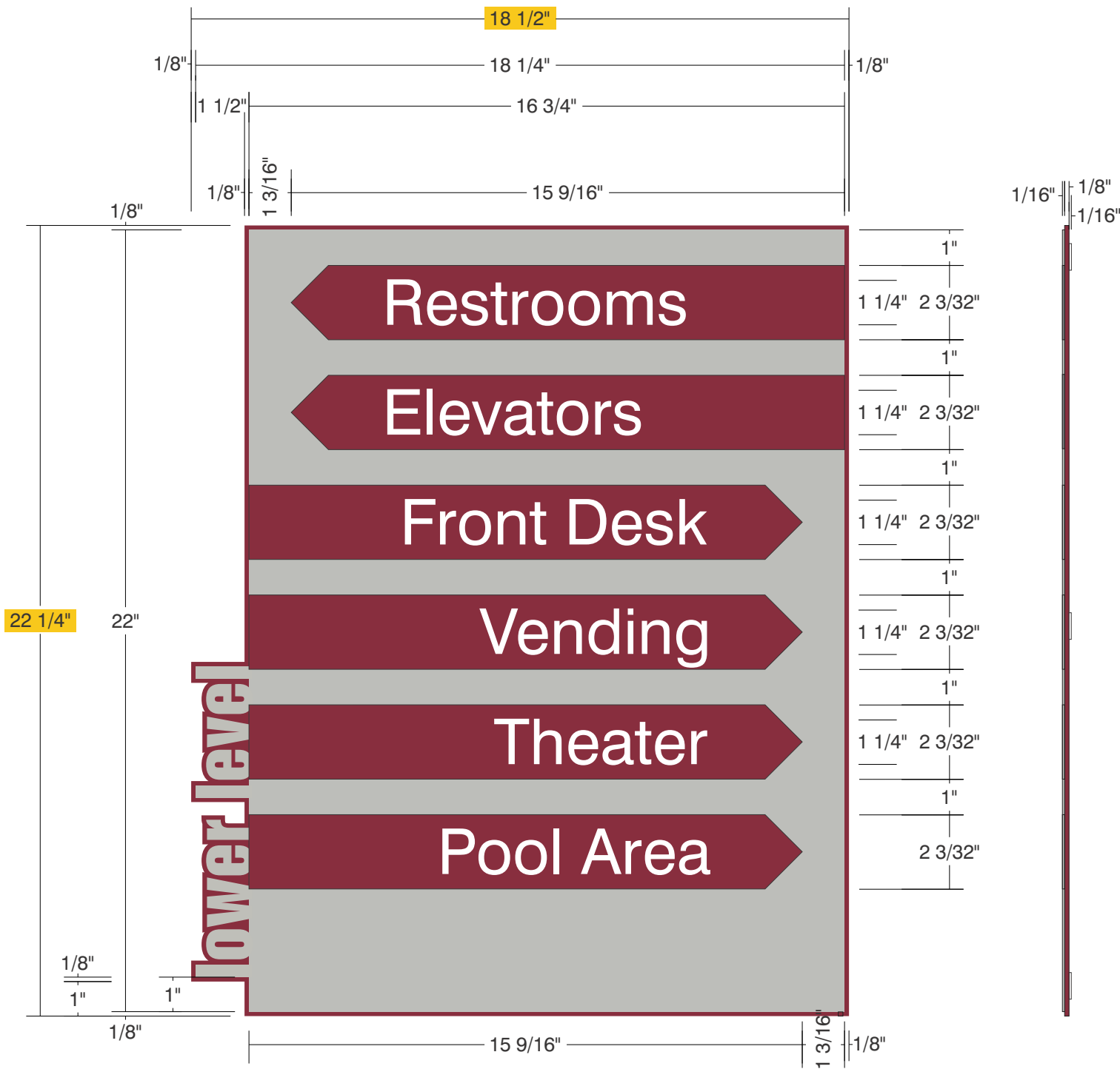
Front View
