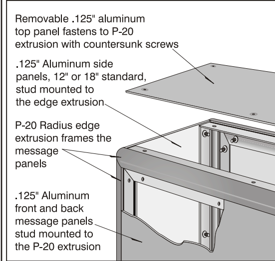
HED P-20 Typical Detail
