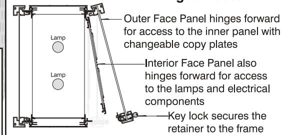
HED I-12 Twin Hinged Faces
