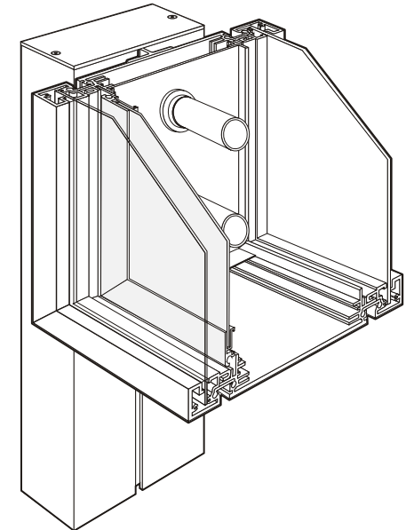
Custom HED I-12 "Twin Hinge" Detail
